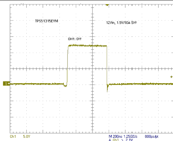
Figure 9-8. Switching Node
