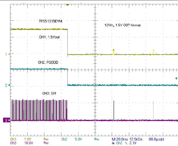
Figure 9-10. Overcurrent Protection (OCP) Hiccup
