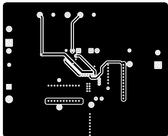
Figure 10-5. Internal Layer 2
