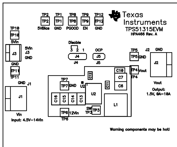
Figure 10-1. Top Layer Assembly Drawing (Top View)
