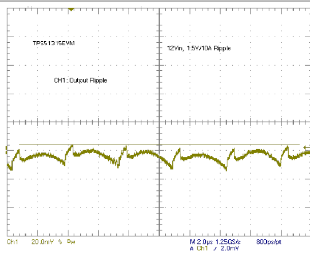
Figure 9-5. Output Ripple
