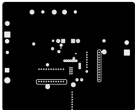
Figure 10-6. Internal Layer 3
