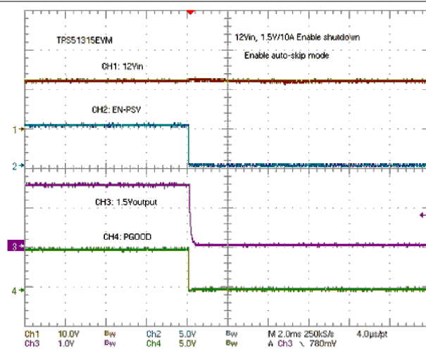
Figure 9-6. Enable Turn-Off
