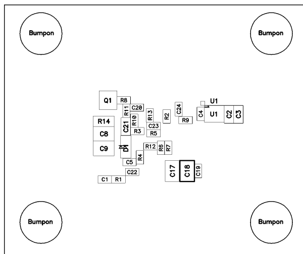
Figure 10-2. Bottom Assembly Drawing (Bottom View)
