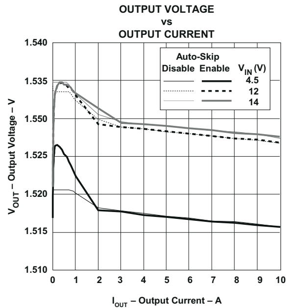
Figure 9-2. TPS51315-EVM Load Regulation
