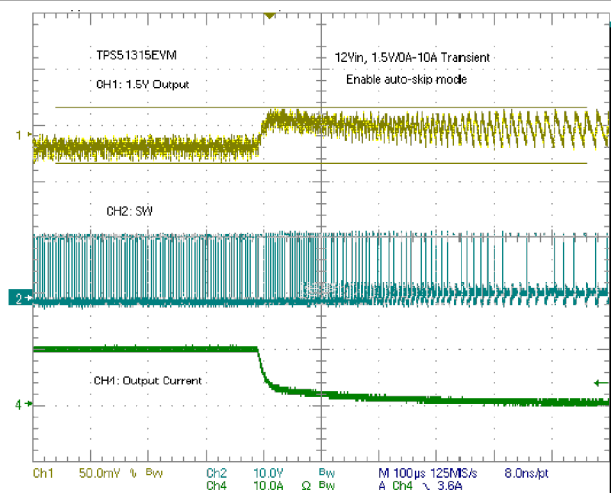
Figure 9-4. 0-A to 10-A Load Transient Fall
