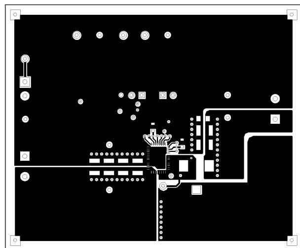
Figure 10-3. Top Copper (Top View)
