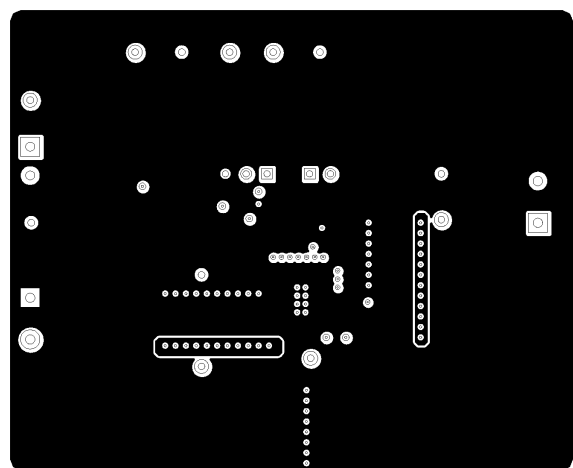
Figure 10-7. Internal Layer 4
