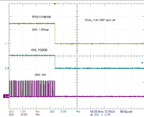
Figure 9-9. Overcurrent Protection (OCP) Latch-Off
