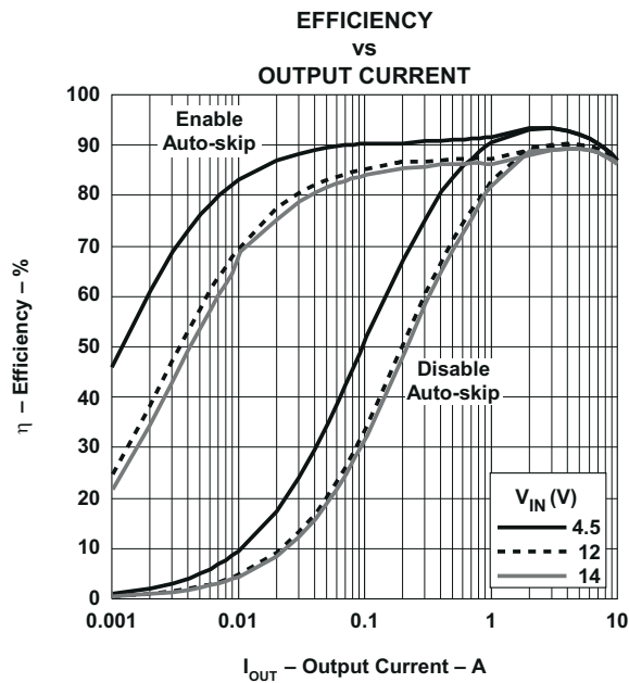
Figure 9-1. TPS51315-EVM Efficiency
