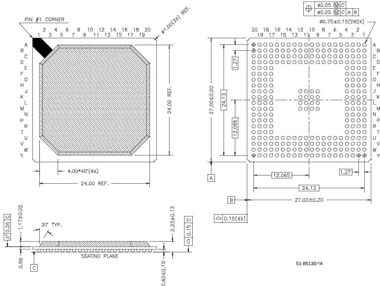
Figure 20-1. Package
