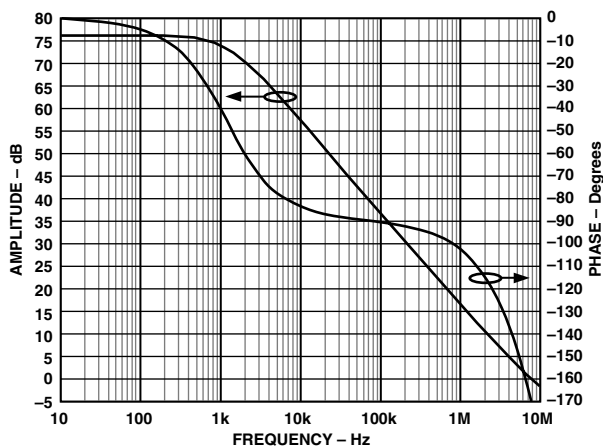
TPC 15. AC Response from VSET to V_{DN}
