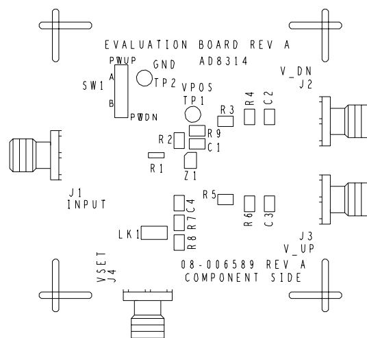
Figure 18. Silkscreen of Component Side (μSO)
