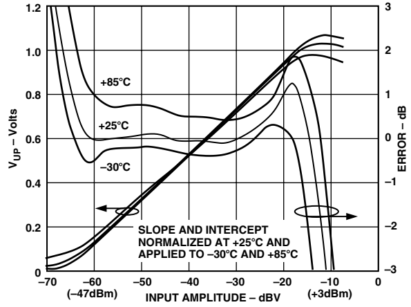
TPC 5. V_{UP} and Log Conformance vs. Input Amplitude at 1.9 GHz; -30°C, +25°C, and +85°C
