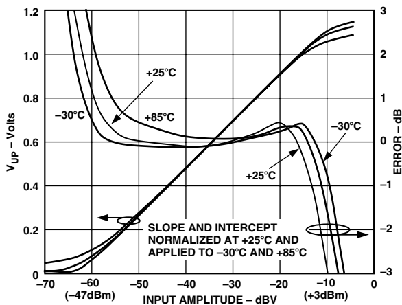
TPC 2. V_{UP} and Log Conformance vs. Input Amplitude at 0.1 GHz; -30°C, +25°C, and +85°C
