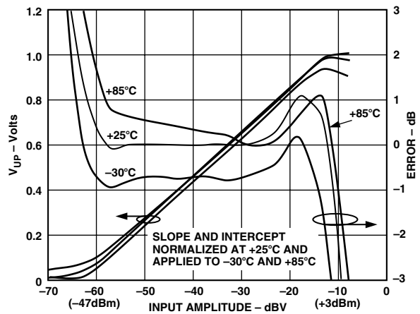
TPC 6. V_{UP} and Log Conformance vs. Input Amplitude at 2.5 GHz; -30°C, +25°C, and +85°C
