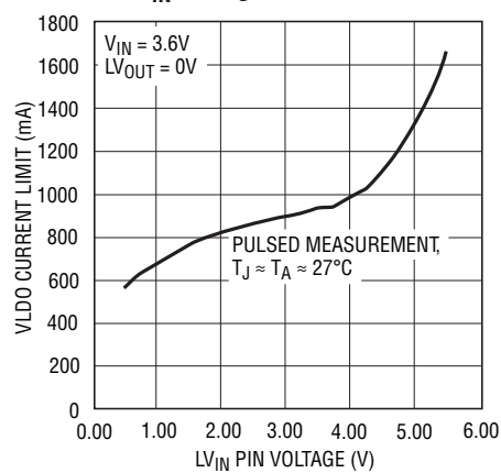
VLDO Current Limit vs LV_{IN} Voltage
