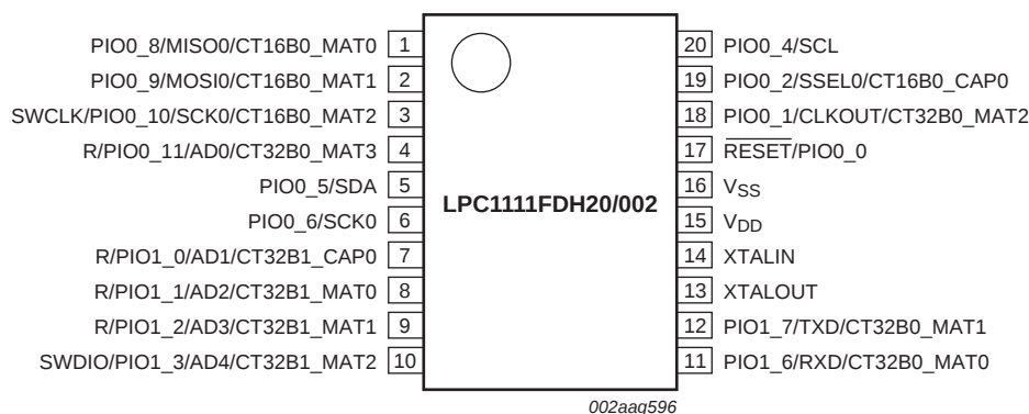
Fig 8. LPC1100L series pin configuration TSSOP20 package with I 2 C-bus pins
