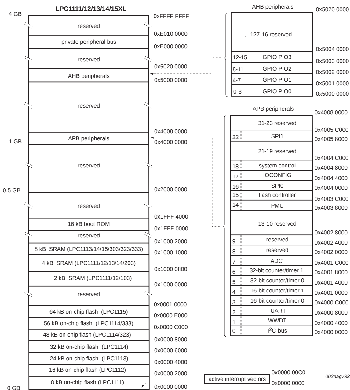
Fig 13. LPC1100XL series memory map
