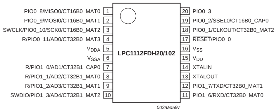
Fig 9. LPC1100L series pin configuration TSSOP20 package with V DDA and V SSA pins
