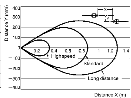
E32-T11R (Through-beam)
