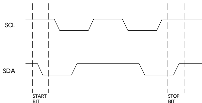
Figure 14: Definition of Start and Stop
