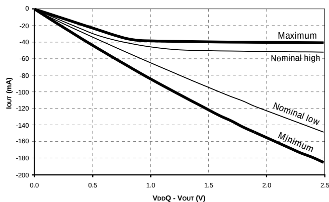
Figure 11: Pull-Up Characteristics
