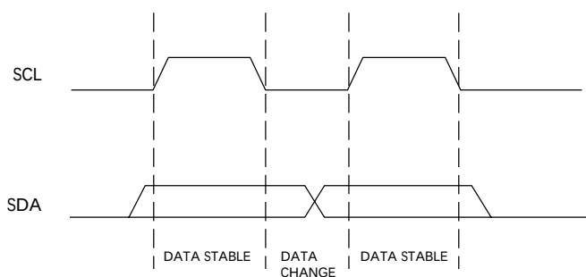
Figure 13: Data Validity
