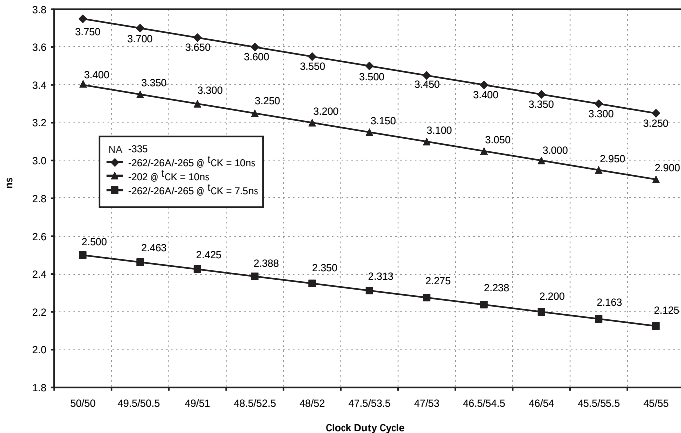
Figure 9: Derating Data Valid Window
