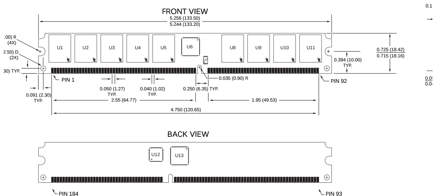
Figure 19: 184-PIN DIMM Dimensions – Very Low-Profile
