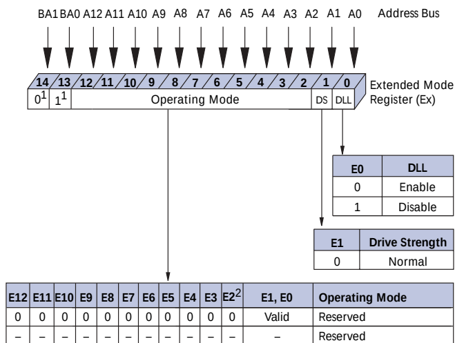
Figure 8: Extended Mode Register Definition Diagram
