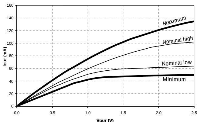
Figure 10: Pull-Down Characteristics
