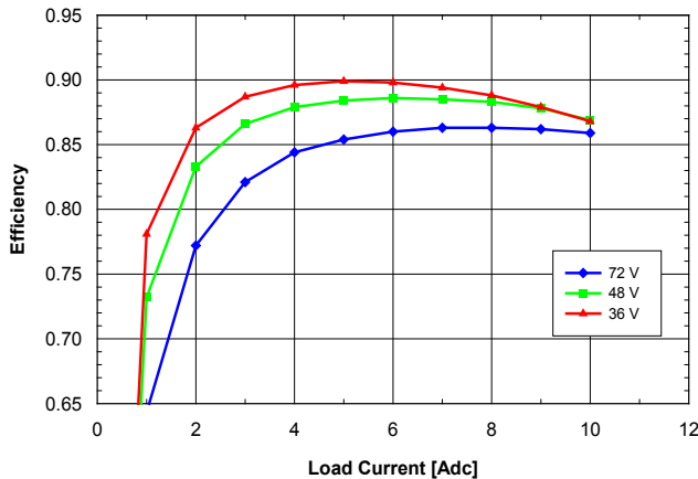
Fig. 5.0V.5: Efficiency vs. load current and input voltage for SQ48T/S10050 converter mounted vertically with air flowing from pin 3 to pin 1 at a rate of 300 LFM (1.5 m/s) and T_a = 25^{\circ}C .
