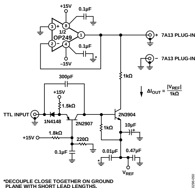
Figure 50. Transient Output Impedance Test Fixture
