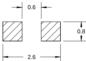
Pad Layout
