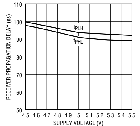
Receiver Propagation Delay vs Supply Voltage
