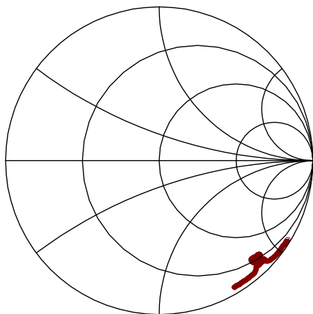
S11 (31.8-41.8 MHz)
