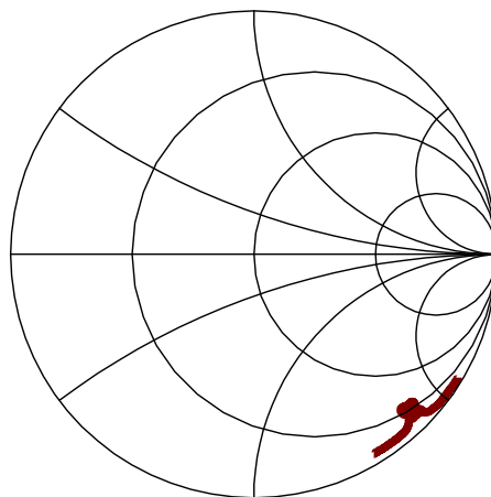
S22 (31.8-41.8 MHz)
