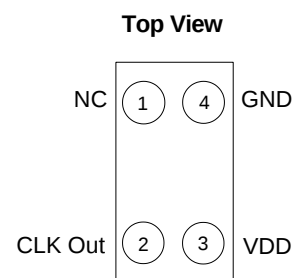
Figure 1. Pin Assignment
