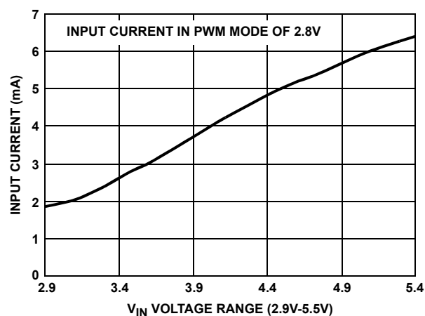
FIGURE 6. I_Q vs V_{IN} (PWM)
