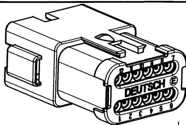
3D VIEW
