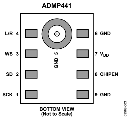
Figure 5. Pin Configuration
