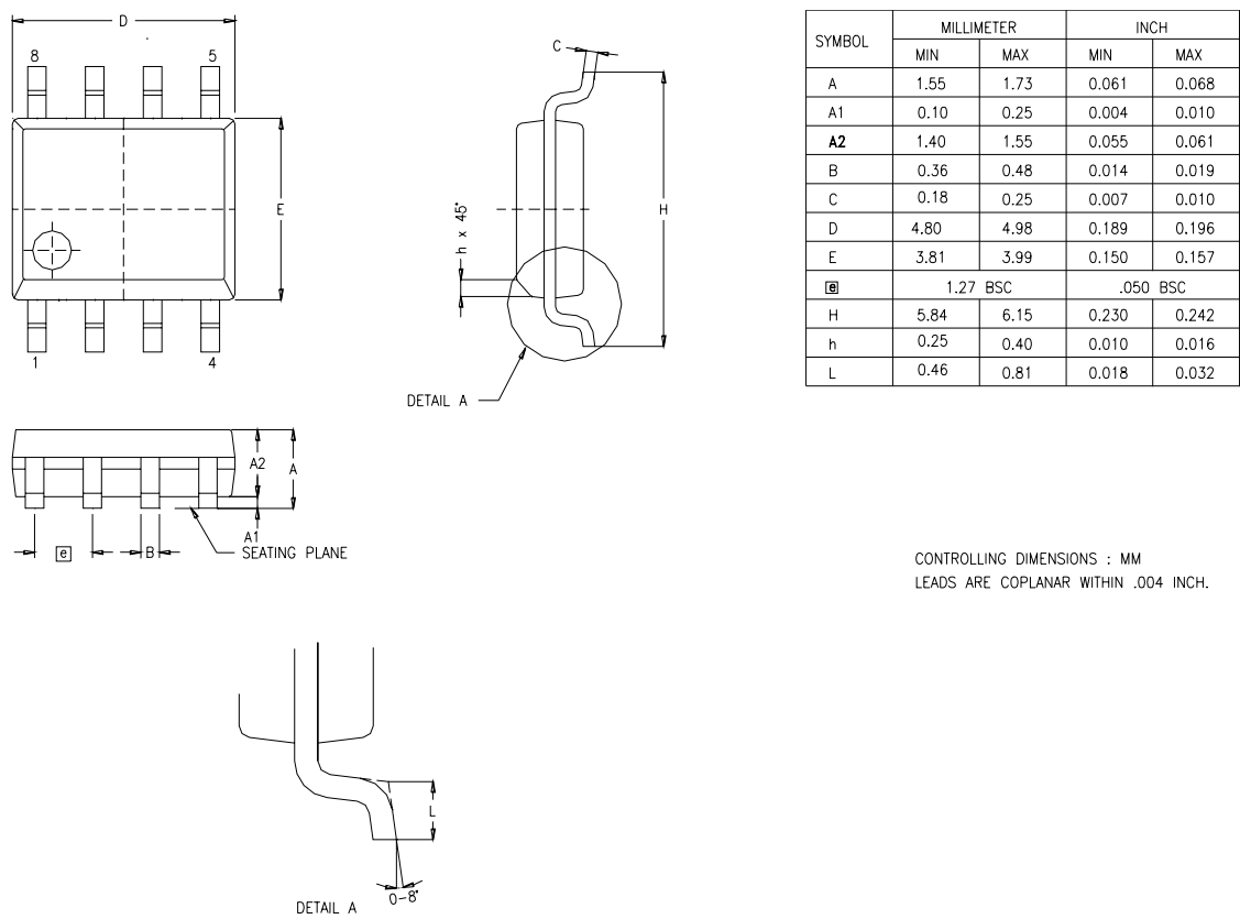
Figure 35. 8-Pin Small Outline Integrated Circuit Package (SOIC)
