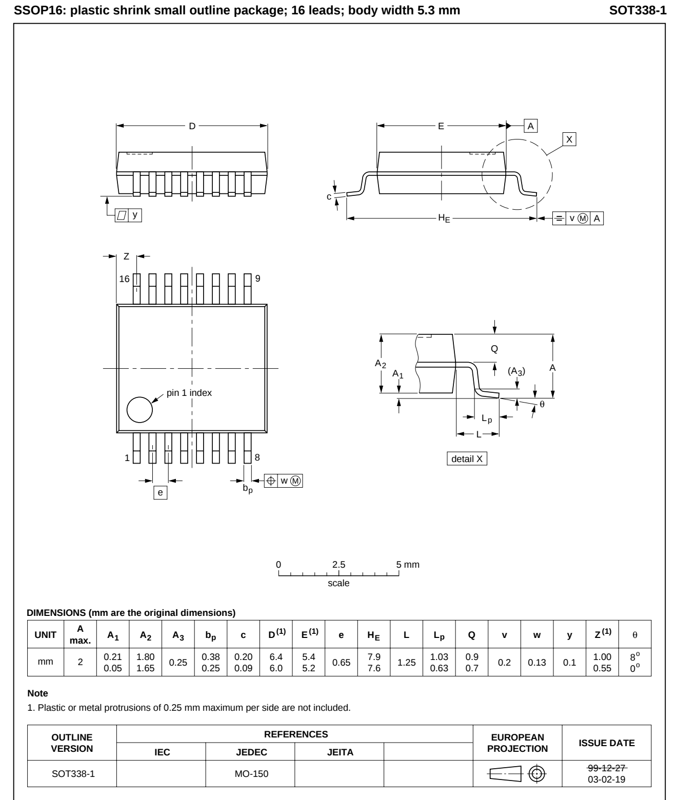
Fig 24. Package outline SOT338-1 (SSOP16)
