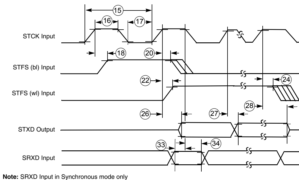
Figure 61. SSI Transmitter External Clock Timing Diagram
