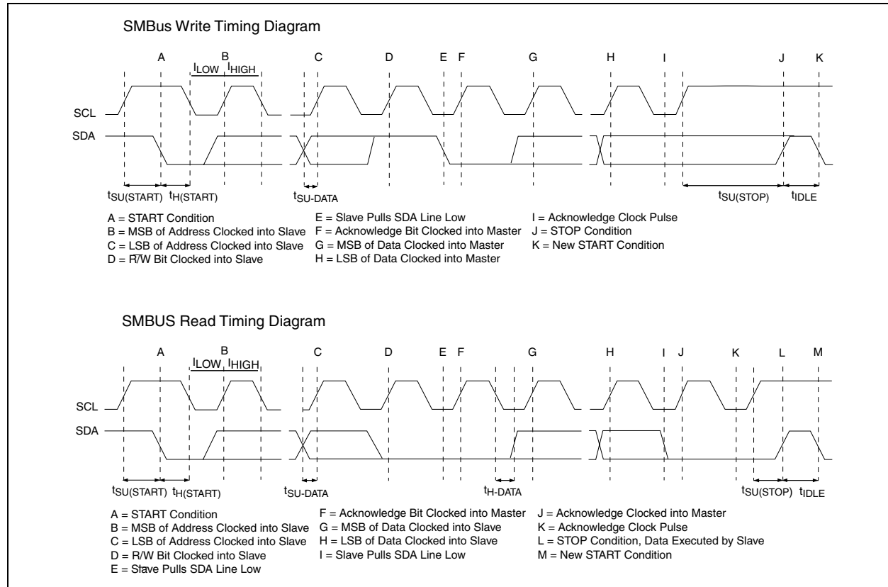
FIGURE 4-1: TIMING DIAGRAMS
