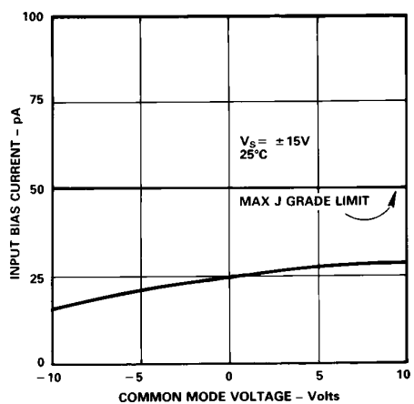
Figure 7. Input Bias Current vs. Common Mode Voltage
