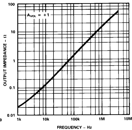
Figure 6. Output Impedance vs. Frequency
