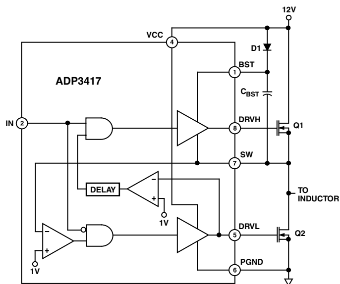
Figure 1. General Application Circuit
