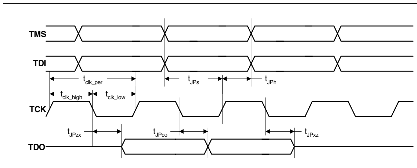
Figure 21. JTAG Timing Measurement
