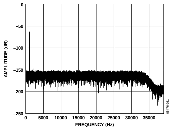
Figure 11. Low Power FFT, 1 kHz, -60 dB Input Tone, 256 \times Decimation
