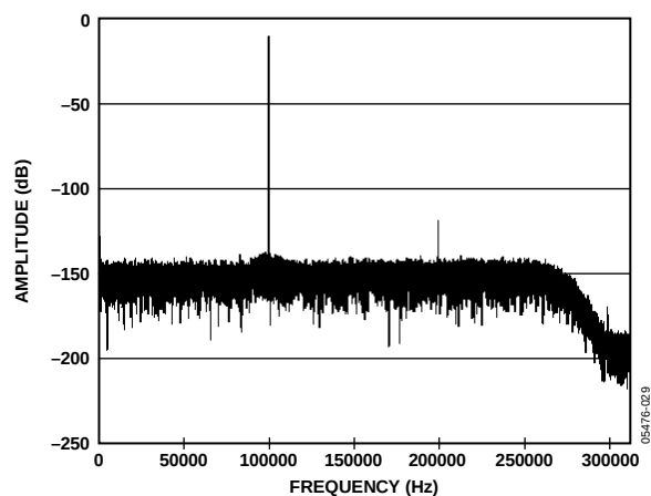
Figure 16. Low Power FFT, 100 kHz, -6 dB Input Tone, 32x Decimation
