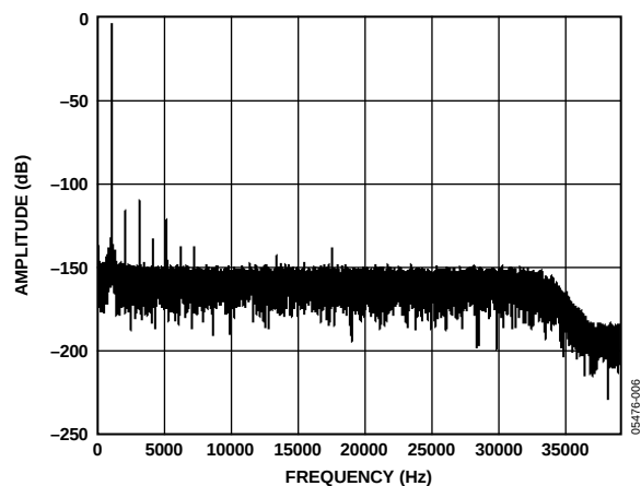
Figure 9. Low Power FFT, 1 kHz, -0.5 dB Input Tone, 256 \times Decimation
