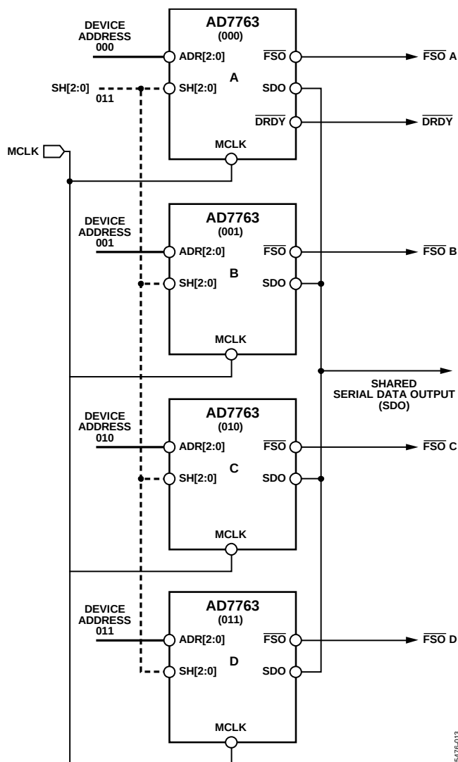
Figure 26. Four AD7763 Devices Sharing the Serial Bus
