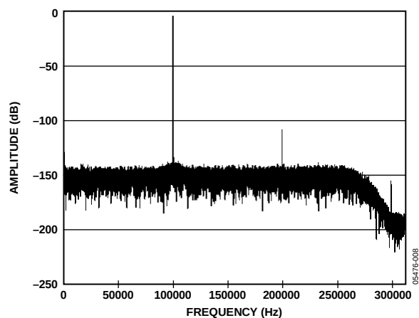
Figure 15. Low Power FFT, 100 kHz, -0.5 dB Input Tone, 32x Decimation
