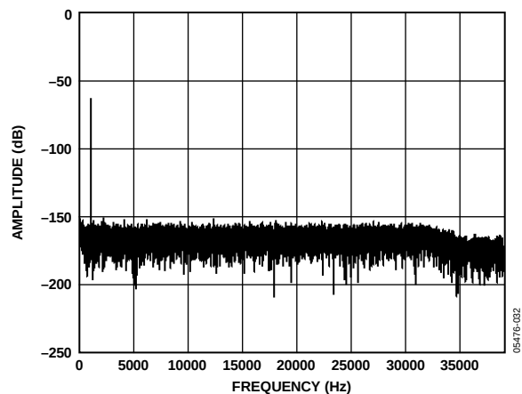
Figure 8. Normal Mode FFT, 1 kHz, -60 dB Input Tone, 256 \times Decimation
