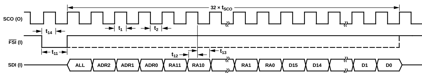
Figure 3. Register Write
