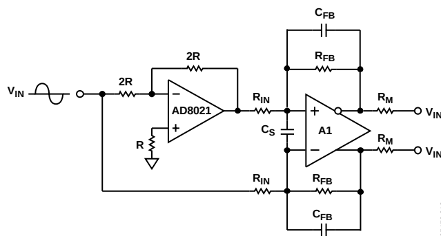
Figure 33. Single-Ended-to-Differential Conversion
