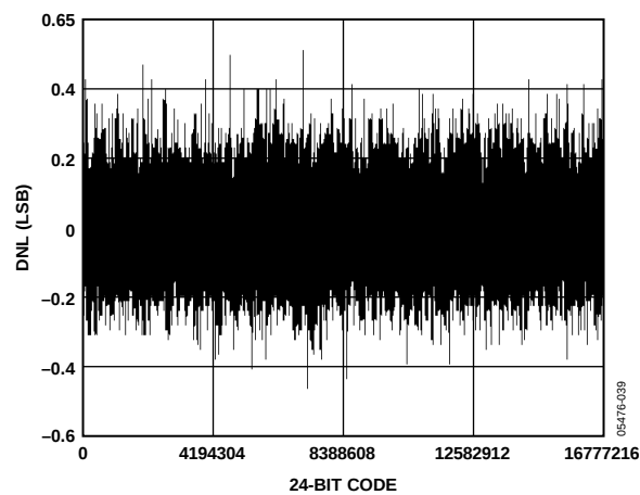
Figure 20. 24-Bit DNL
