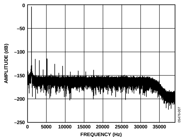
Figure 6. Normal Mode FFT, 1 kHz, -0.5 dB Input Tone, 256 \times Decimation
