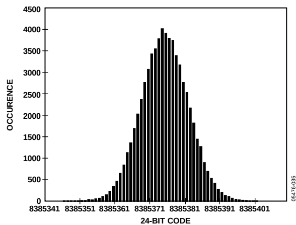
Figure 18. Normal Mode, 24-Bit Histogram, 256× Decimation
