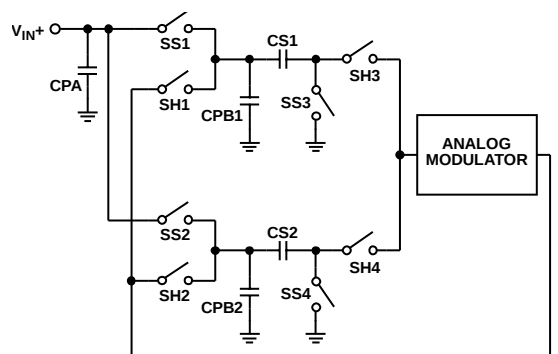
Figure 34. Equivalent Input Circuit
