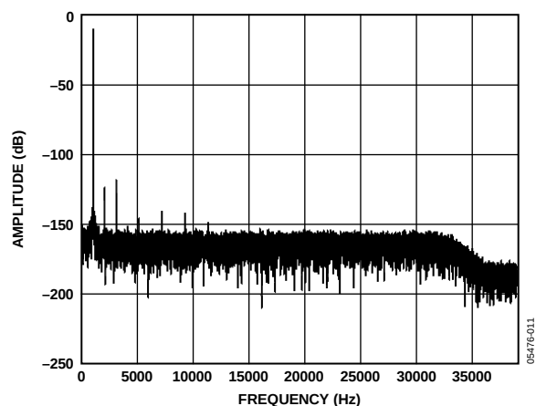
Figure 7. Normal Mode FFT, 1 kHz, -6 dB Input Tone, 256 \times Decimation
