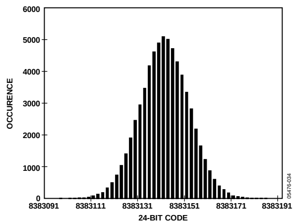
Figure 21. Low Power 24-Bit Histogram, 256× Decimation
