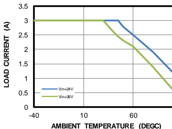
Thermal Derating
