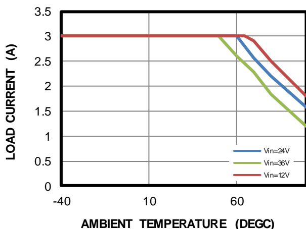
Thermal Derating
