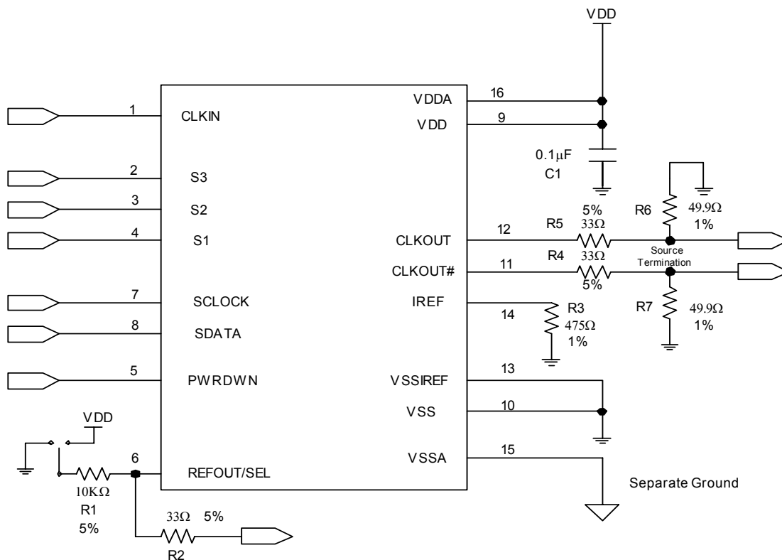
Figure 4. Application Schematic
