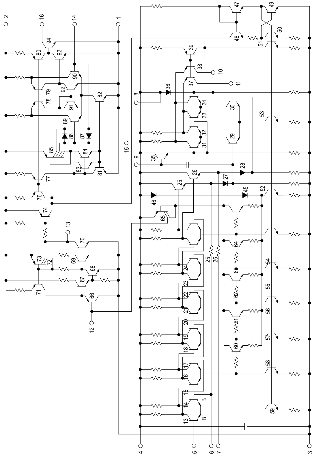
Figure 15. Internal Schematic
