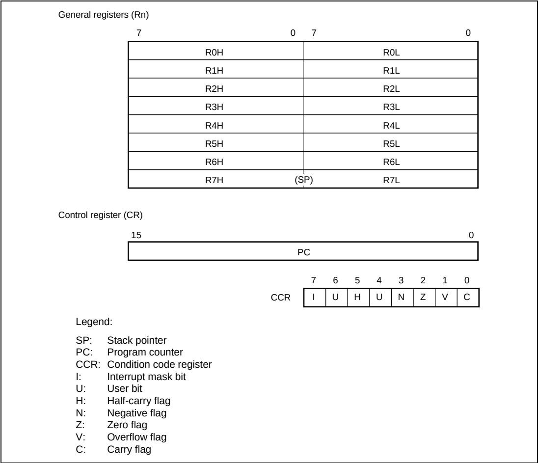
Figure 2.2 CPU Registers
