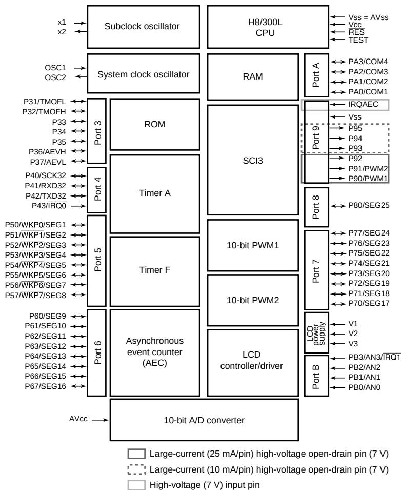
Figure 1.1 Internal Block Diagram of H8/3802 Group
