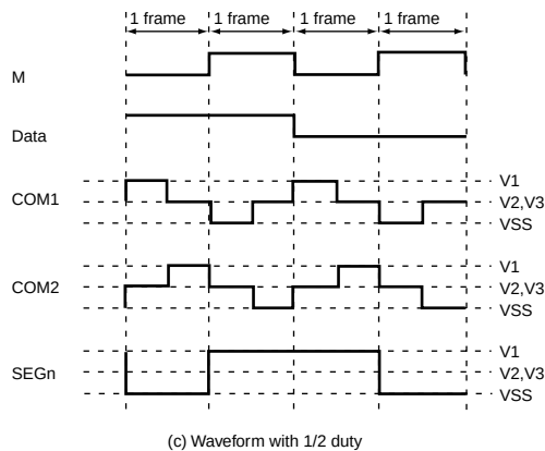
(c) Waveform with 1/2 duty
