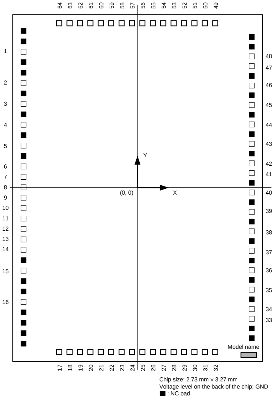
Figure 1.8 Pad Arrangement of HCD64338004, HCD64338003, HCD64338002, HCD64338001, and HCD64338000 (Top View)
