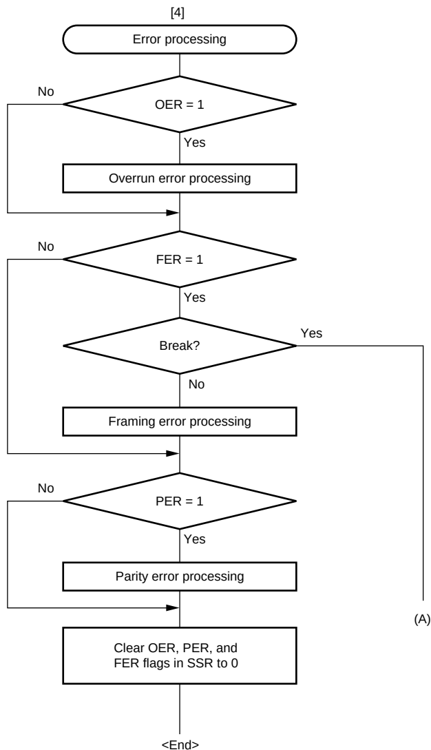
Figure 10.8 Sample Serial Data Reception Flowchart (Asynchronous Mode) (2)
