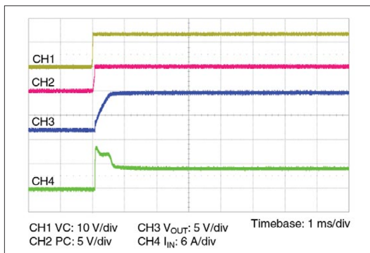
Figure 11 — Start up from application of VC; V_{IN} pre-applied C_{OUT} = 2300 \mu F
