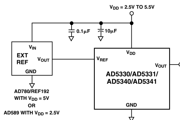
Figure 34. AD5330/AD5331/AD5340/AD5341 Using External Reference
