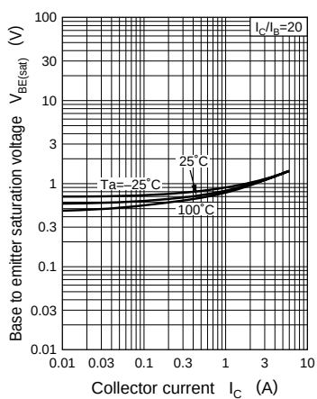
V_{BE(\text{sat})} - I_C
