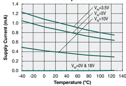
Quiescent Supply Current vs. Temperature
