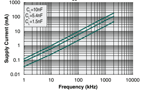
Supply Current vs. Frequency ( V_{CC}=8V )
