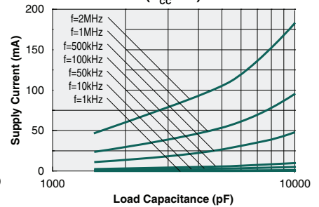
Supply Current vs. Load Capacitance ( V_{CC}=8V )
