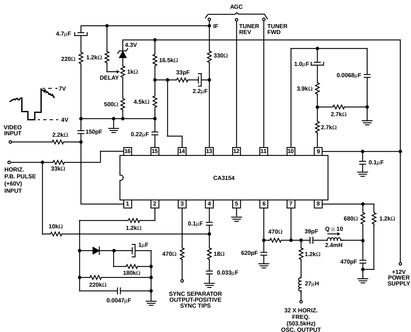
FIGURE 7. TYPICAL APPLICATION OF THE CA3154
