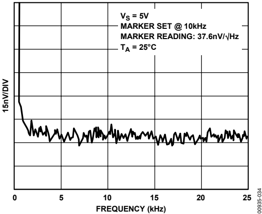
Figure 34. Voltage Noise
