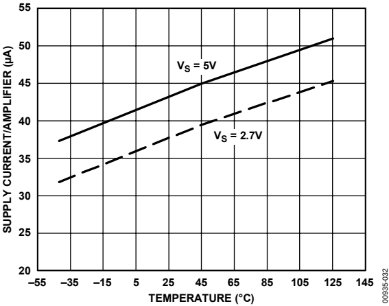
Figure 32. Supply Current per Amplifier vs. Temperature
