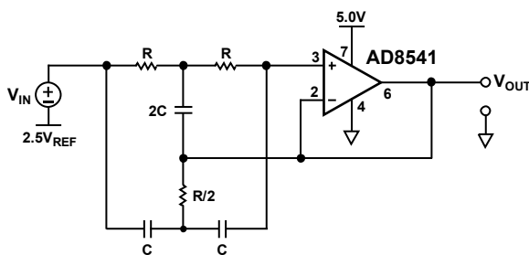
Figure 36. 60 Hz Twin-T Notch Filter, Q = ∞ (Ideal)
