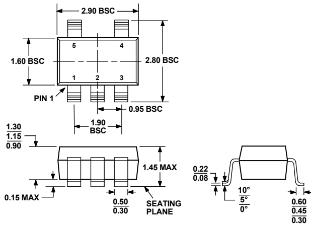
Figure 40. 5-Lead Small Outline Transistor Package [SOT-23]
