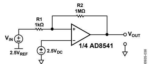
Figure 38. AD854x Comparator Application—Overload Detector
