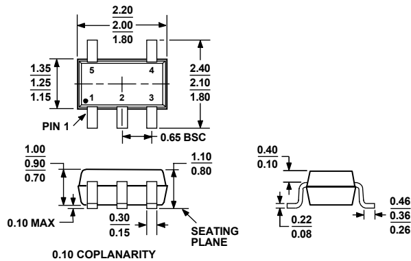
Figure 42. 5-Lead Thin Shrink Small Outline Transistor Package [SC70]
