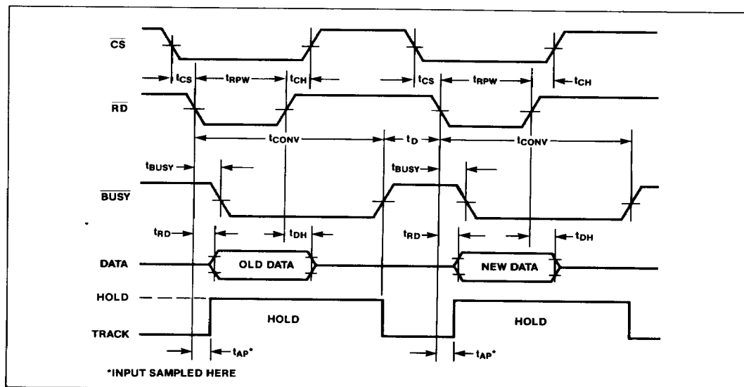
Figure 13. Timing Diagram—ROM Mode
