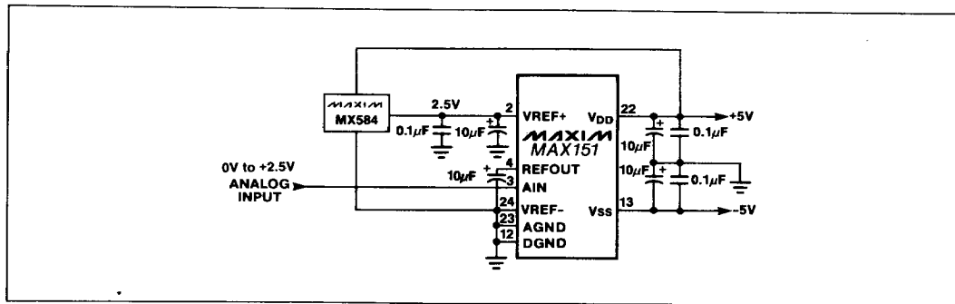
Figure 8. External Reference 2.5V Full-Scale
