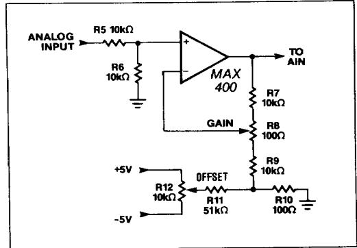
Figure 11. Offset ( \pm 20\text{mV} ) and Gain ( \pm 0.5\% ) Trim Circuit
