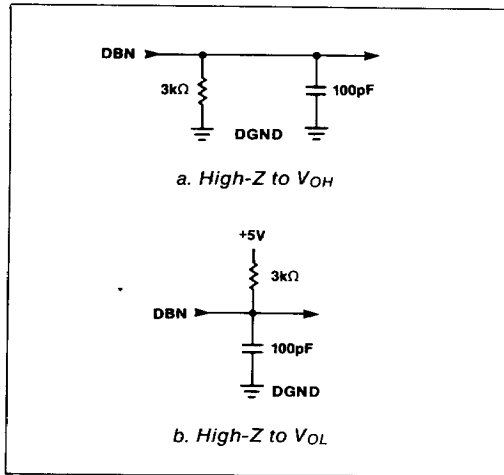
Figure 1. Load Circuits for Data Access Time Test
