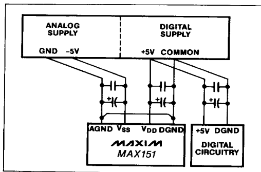
Figure 14. Power-Supply Grounding Practice
