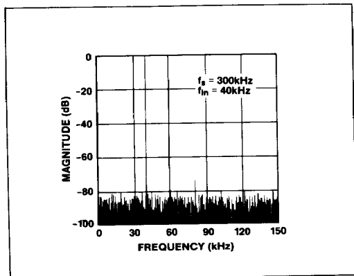
Figure 15. FFT Plot for the MAX151
