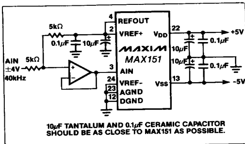
Figure 4. \pm 4V Bipolar Input with Driving Amplifier
