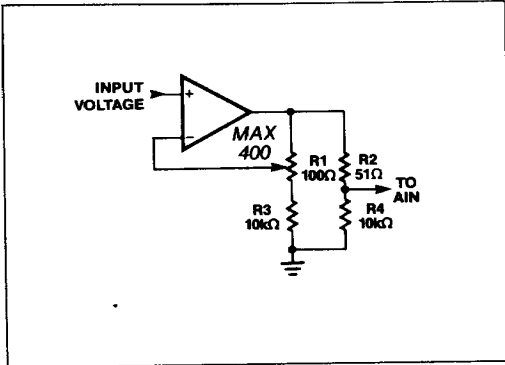
Figure 10. Trim Circuit for Full-Scale Only ( \pm 0.5\% )
