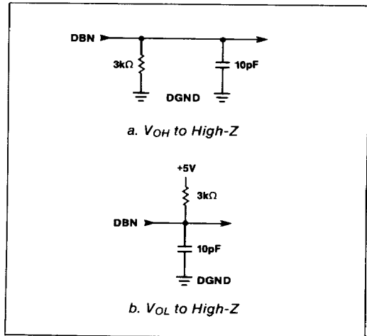
Figure 2. Load Circuits for Bus Relinquish Time Test
