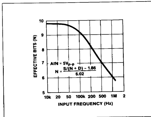
Figure 16. Effective Bits Curve
