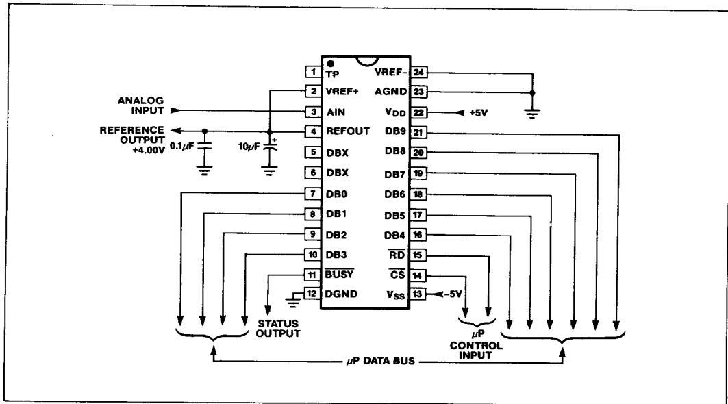
Figure 3. MAX151 Operational Diagram
