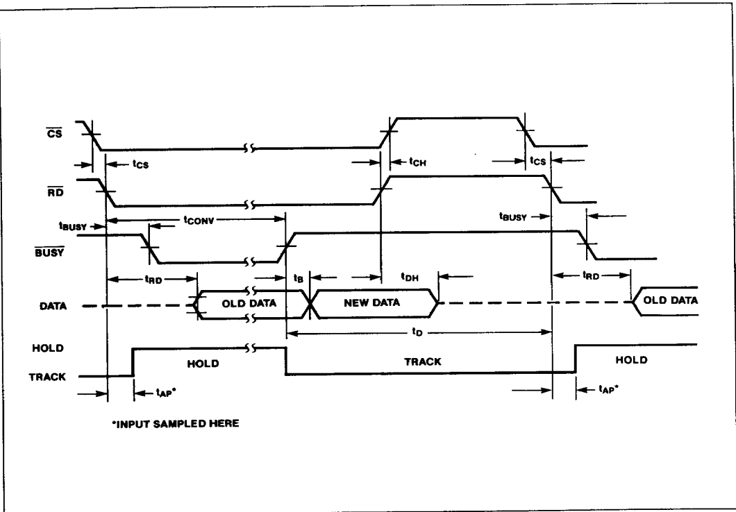
Figure 12. Timing Diagram—Slow Memory Mode
