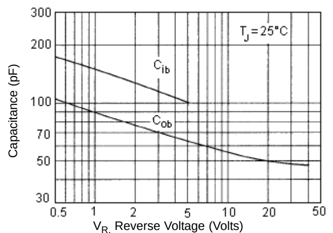
Capacitances
