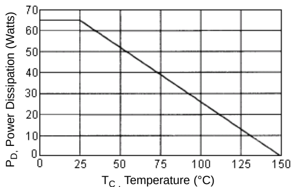
Power Derating
