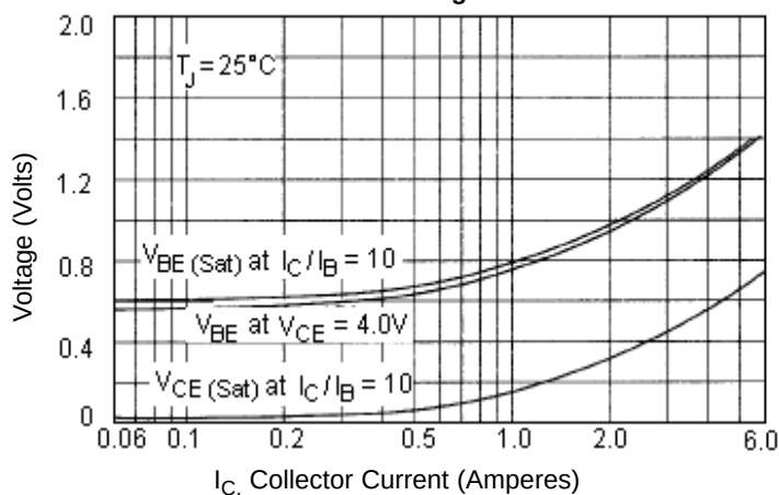
"ON" Voltage
