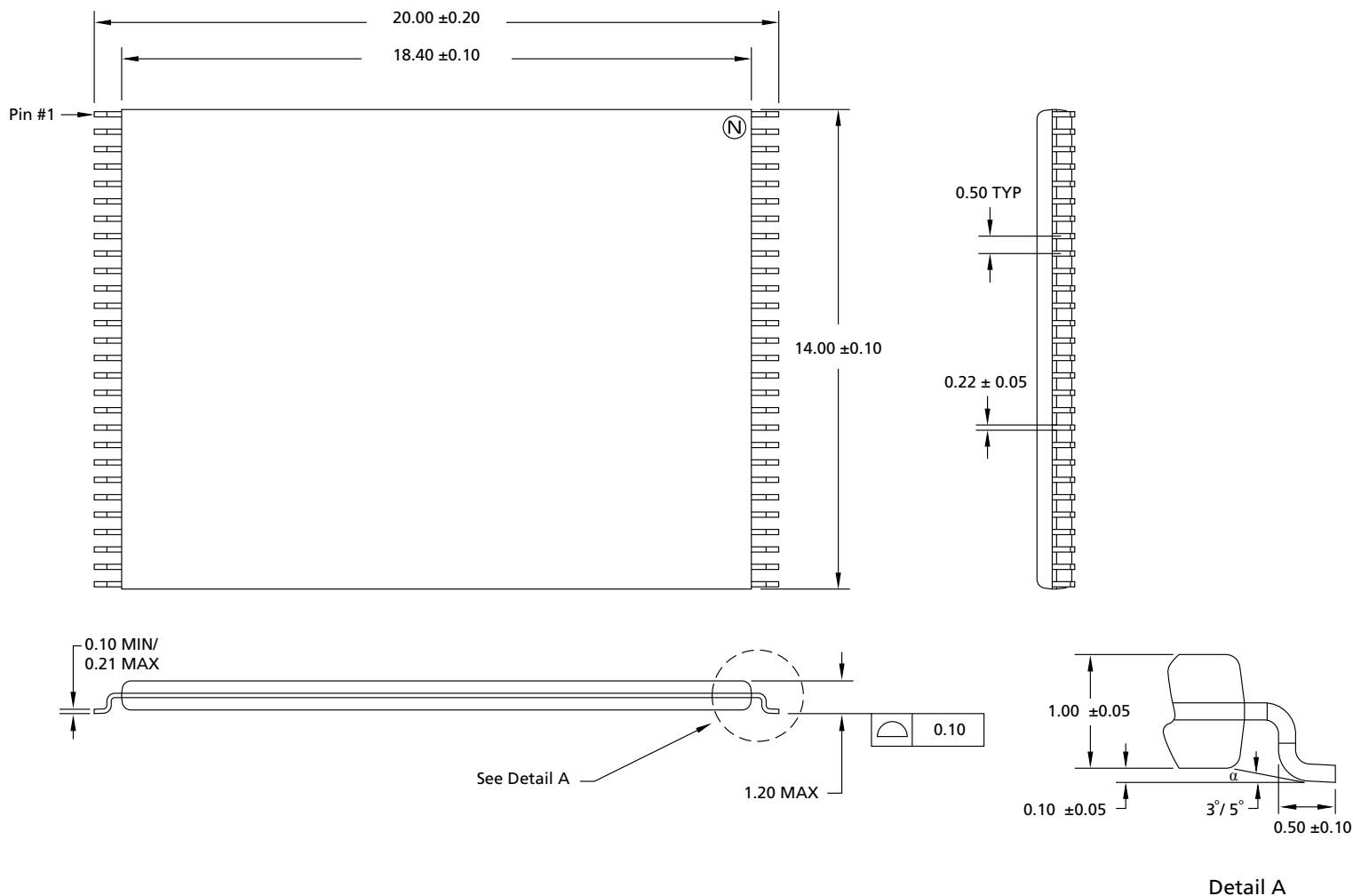
Figure 31: 56-Pin TSOP – 14mm x 20mm
