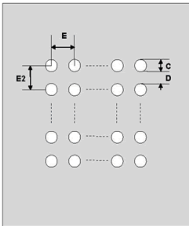
Top View (SMT Footprint)
