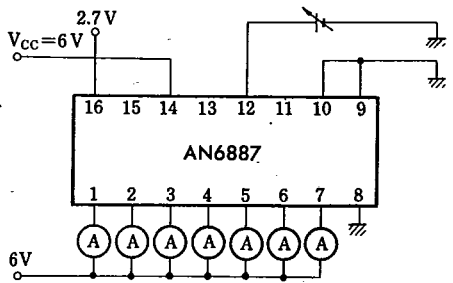
Test Circuit 7 ( I_{(SINK)1-7} )
