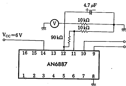
Test Circuit 5 ( V_{O(\text{offset})} )
