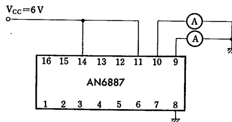
Test Circuit 4 ( I_{Bias12} )
