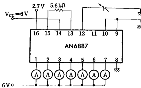
Test Circuit 8 ( I_{(SINK)1\sim7} , GD_{1\sim7} )
