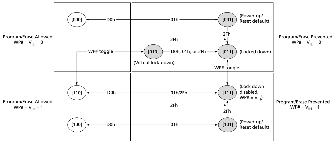
Figure 8: Block Locking State Diagram
