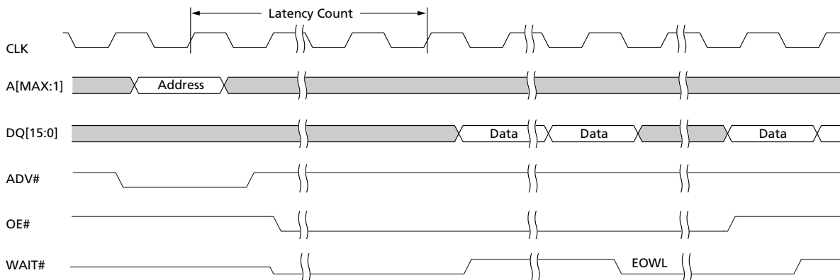
Figure 11: End of Wordline Timing Diagram
