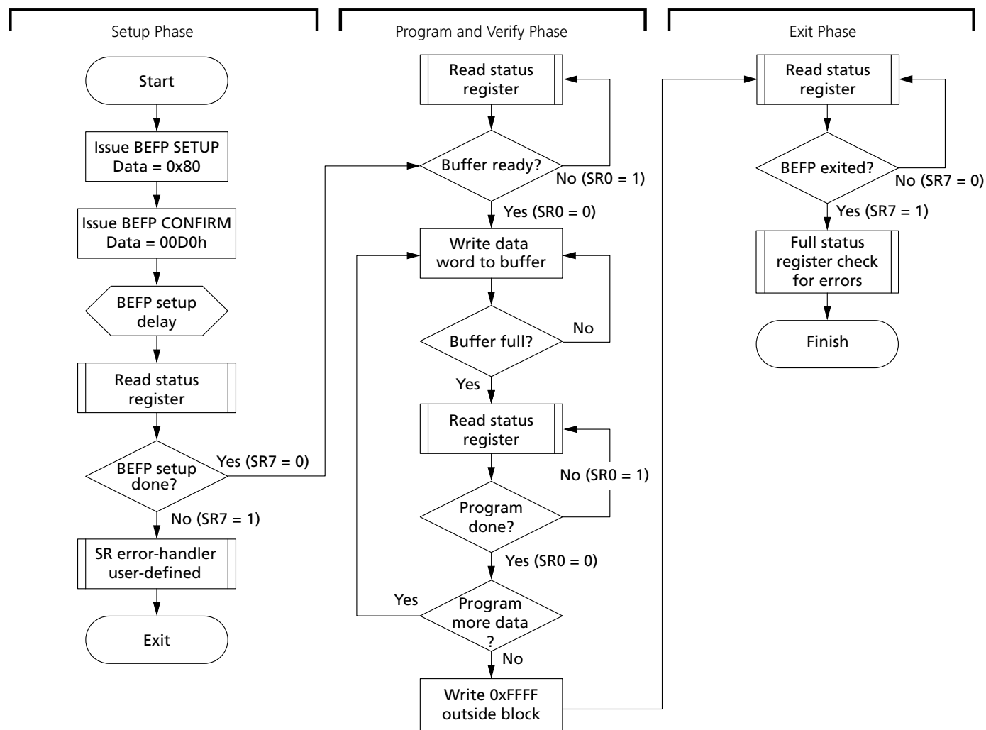
Figure 15: Buffered Enhanced Factory Programming (BEFP) Procedure
