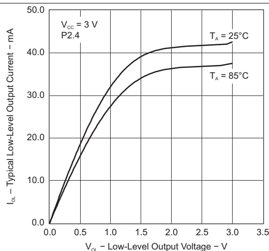
Figure 16. Typical Low-Level Output Current vs Low-Level Output Voltage
