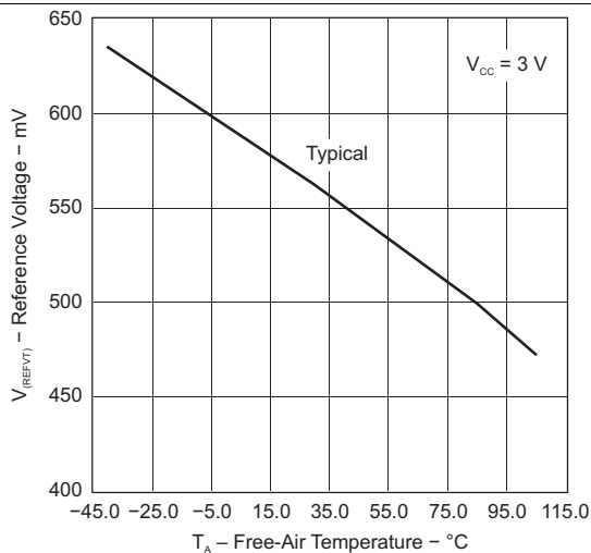
Figure 29. V_{(RefVT)} vs Temperature V_{CC} = 2.2\text{ V}
