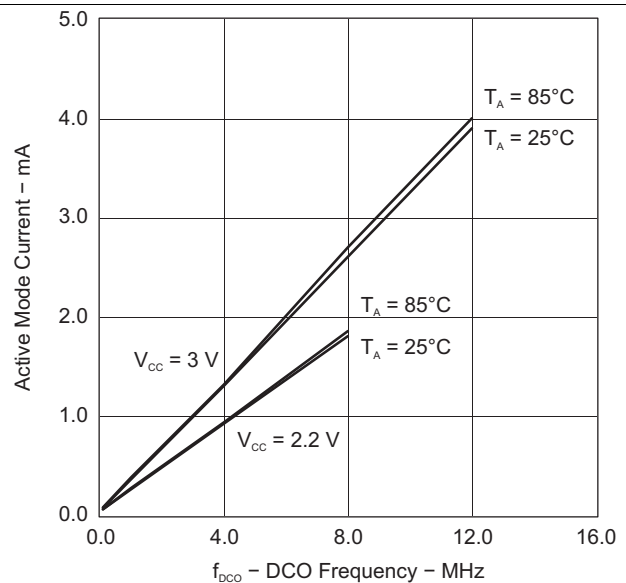
Figure 13. Active-Mode Current vs DCO Frequency
