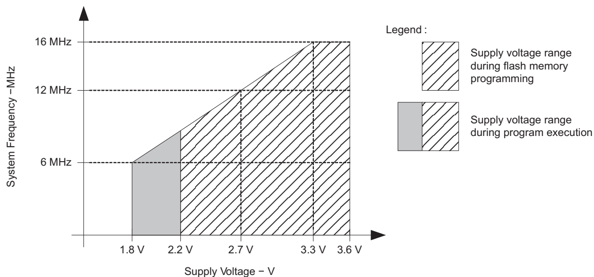
Figure 2. Operating Area
