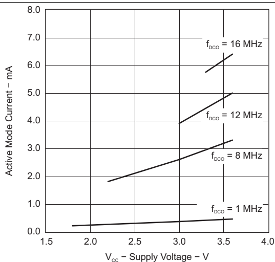
Figure 12. Active-Mode Current vs Supply Voltage T A = 25°C
