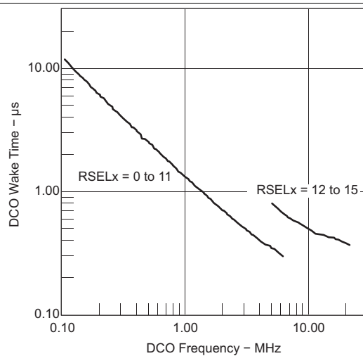
Figure 22. Clock Wake-Up Time From LPM3 vs DCO Frequency
