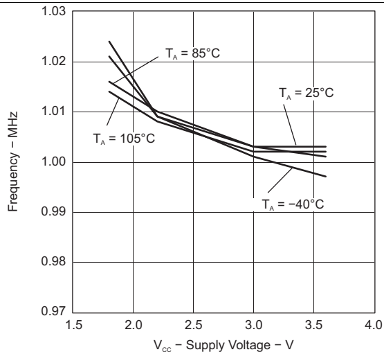
Figure 21. Calibrated 1-MHz Frequency vs Supply Voltage
