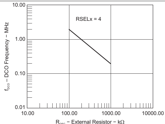
Figure 24. DCO Frequency vs R_{OSC} V_{CC} = 3 V, T_A = 25^\circ\text{C}
