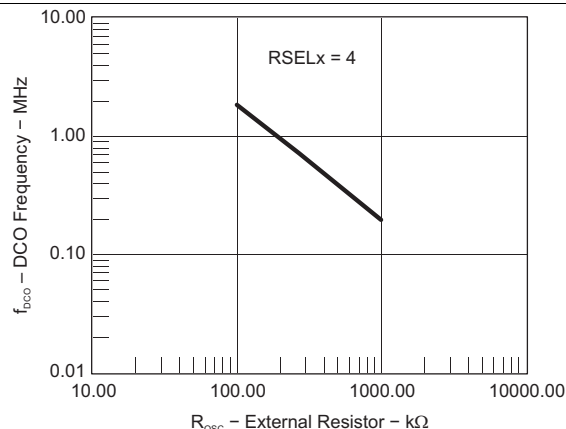
Figure 23. DCO Frequency vs R_{OSC} V_{CC} = 2.2 V, T_A = 25^\circ\text{C}
