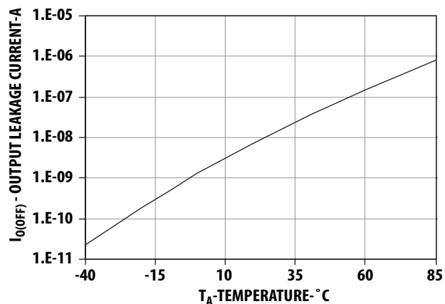
Figure 4. Typical Output Leakage vs Ambient Temperature
