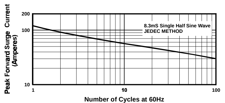
FIGURE 6. MAXIMUM NON-REPETITIVE PEAK FORWARD SURGE CURRENT - UNIDIRECTIONAL
