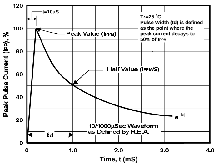
FIGURE 3. PULSE WAVEFORM
