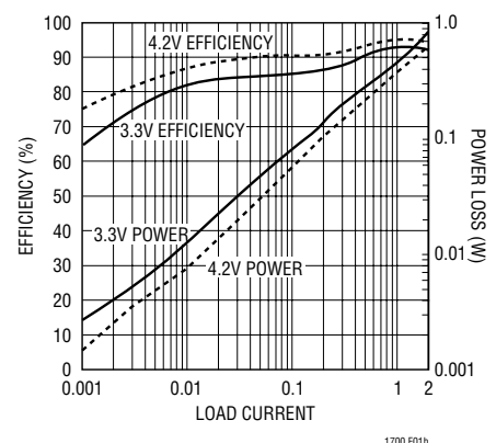
Efficiency, Power Loss vs Load Current
