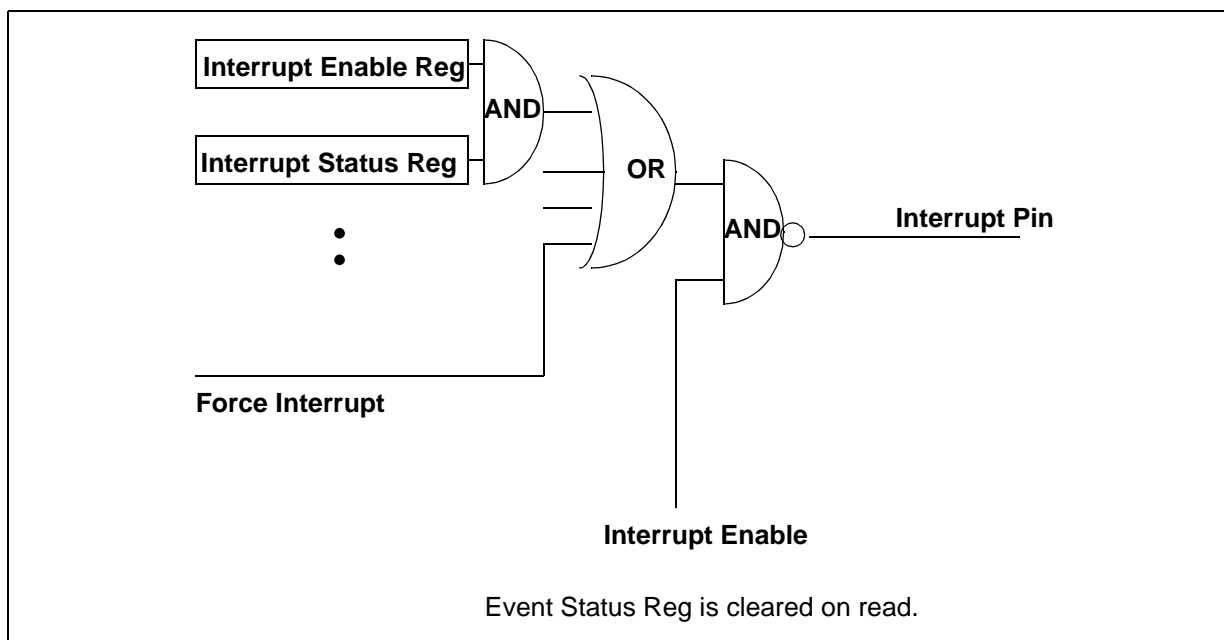
Figure 13. Interrupt Handling
