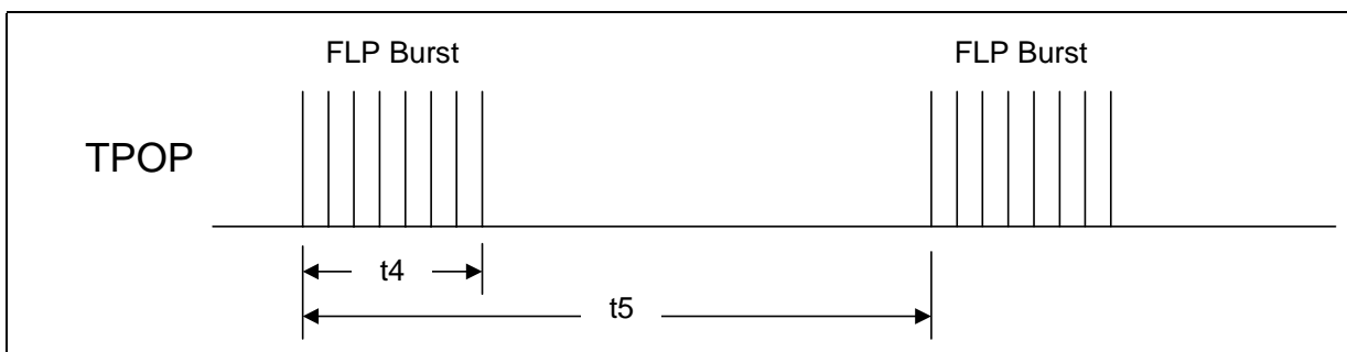
Figure 54. FLP Burst Timing
