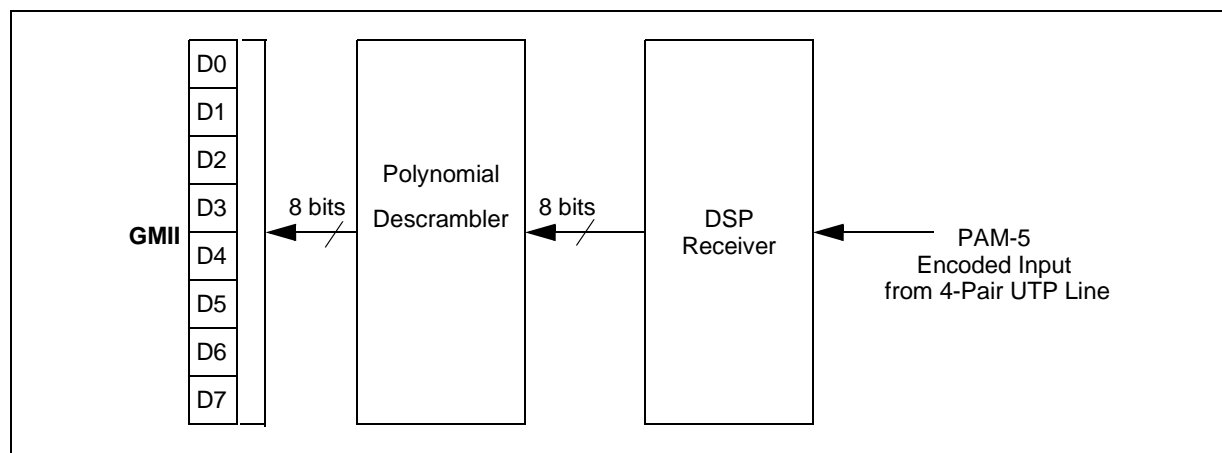
Figure 20. 1000BASE-T Receive Flow
