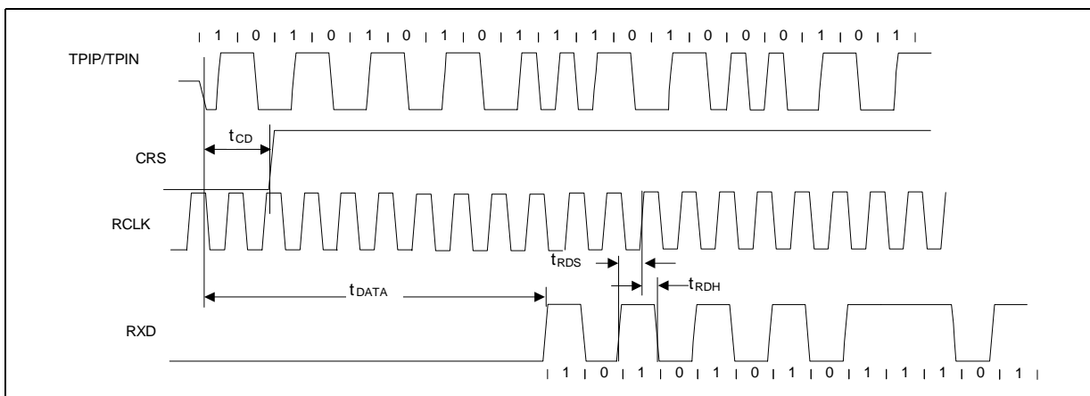
Figure 51. 10BASE-T Serial Start-of-Frame Timing
