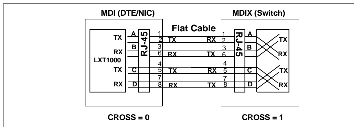
Figure 5. Crossover Function
