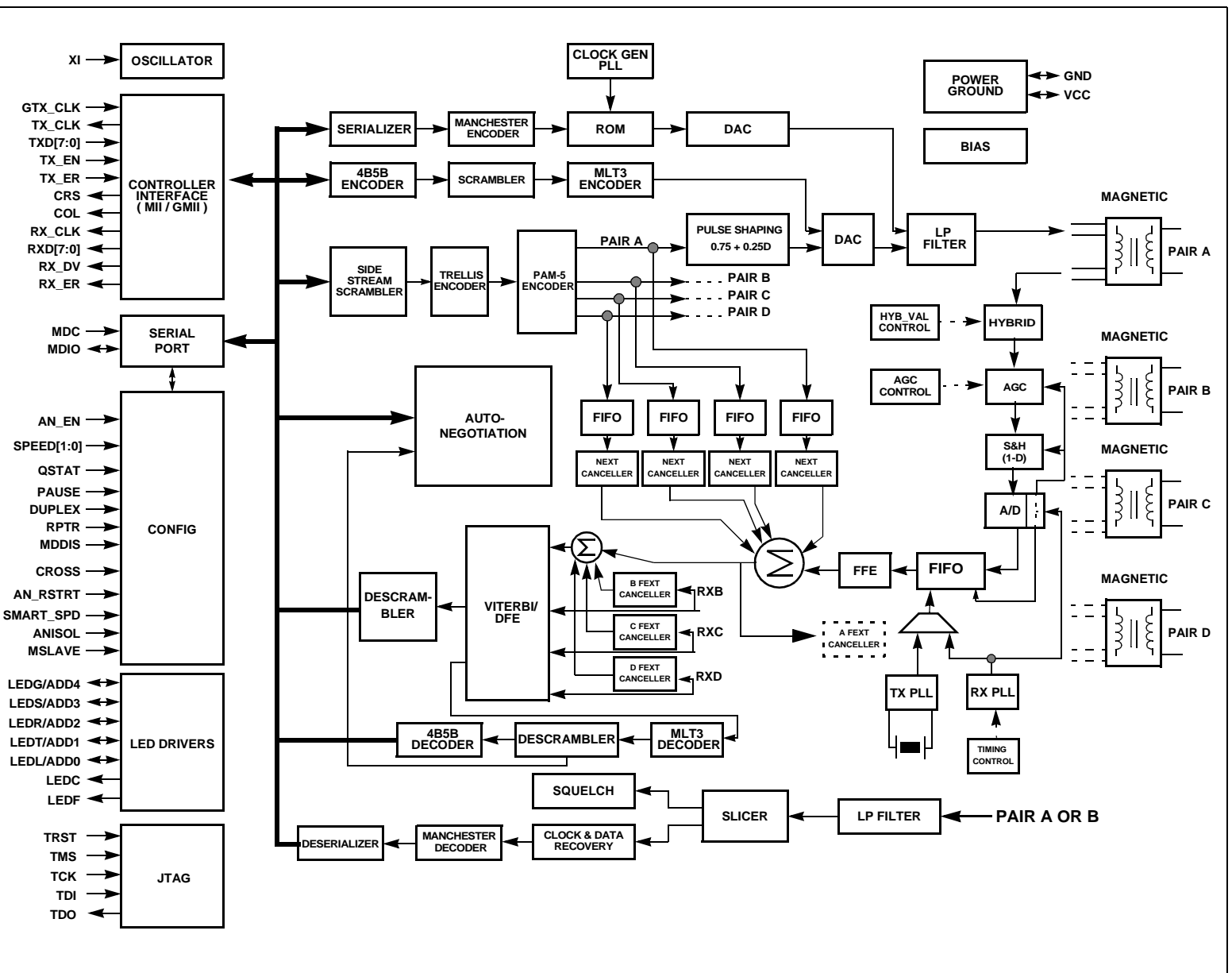
Figure 4. LX1000 Block Diagram
