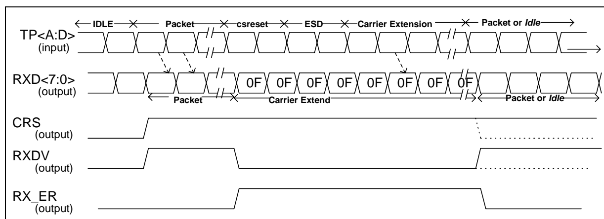
Figure 29. 1000BASE-T Reception, Carrier Extension and Packet Concatenation
