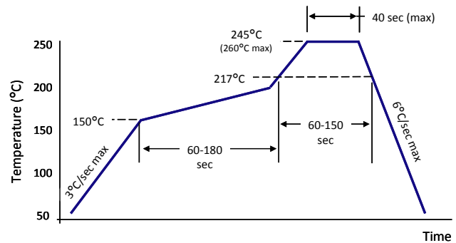
Solder Reflow Profile
