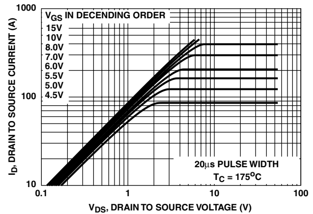
FIGURE 2. OUTPUT CHARACTERISTICS
