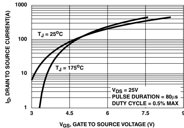
FIGURE 3. TRANSFER CHARACTERISTICS
