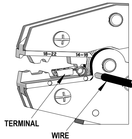
POSITION FOR 14-16 TERMINALS
