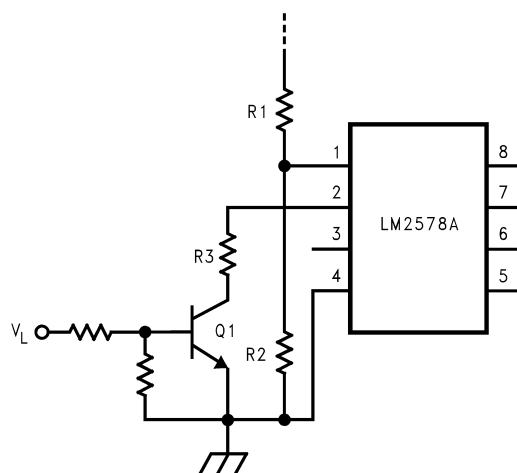
FIGURE 11. Shutdown Occurs when V_L is High
