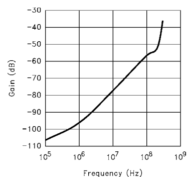
FIGURE 18. CHANNEL-CHANNEL ISOLATION
