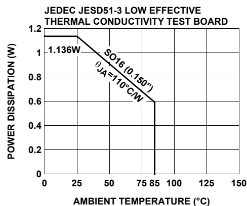
FIGURE 24. POWER DISSIPATION vs AMBIENT TEMPERATURE
